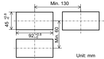
Panel cutout
