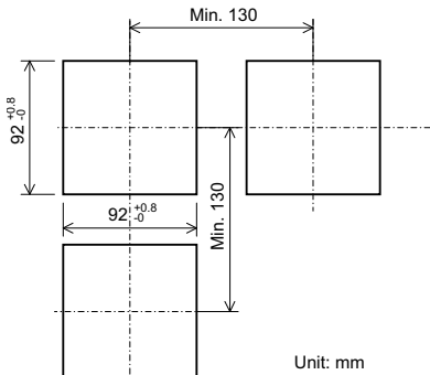
Panel cutout
